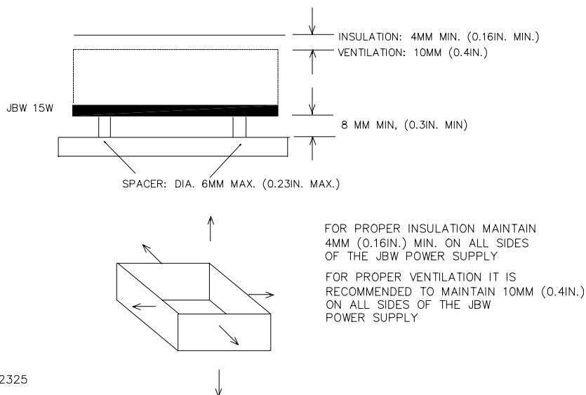
FIGURE 3. VENTILATION AND INSULATION
