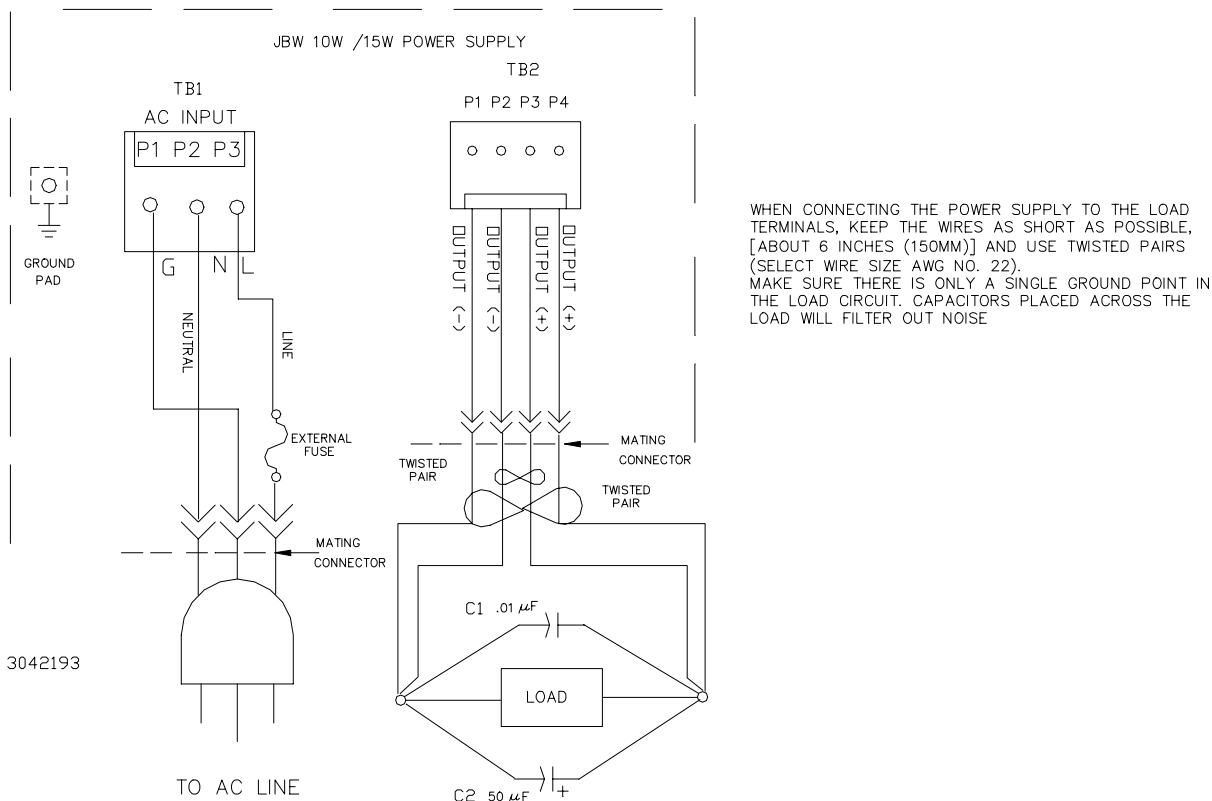
FIGURE 2. LOAD CONNECTIONS
