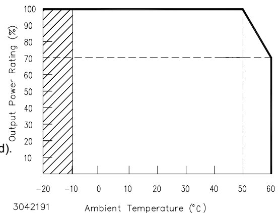
FIGURE 1. DERATING PLOT
